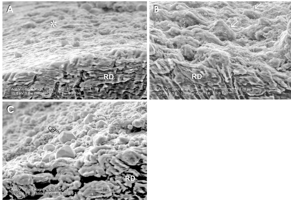
Figure 3. Representative ESEM images taken from the gutta-percha/AH Plus group following dislodging of the root fillings with the thin-slice push-out test. (A) An overall view of a characteristic type of interfacial failure that occurred by the detachment of the gutta-percha, with remnant epoxy resin sealer (asterisk) over the surface of the intraradicular dentin. RD: sectioned surface of the root dentin slice. (B) A higher magnification view, showing blebs of remnant resin sealer (arrows) that projected into the space previously occupied by the unbonded gutta-percha. (C) Crystalline structures (pointer) that represent large, remnant fillers (probably zirconium oxide or calcium tungstate—AH Plus, MSDS data) derived from the AH Plus resin sealer. RD: root dentin slice surface.
