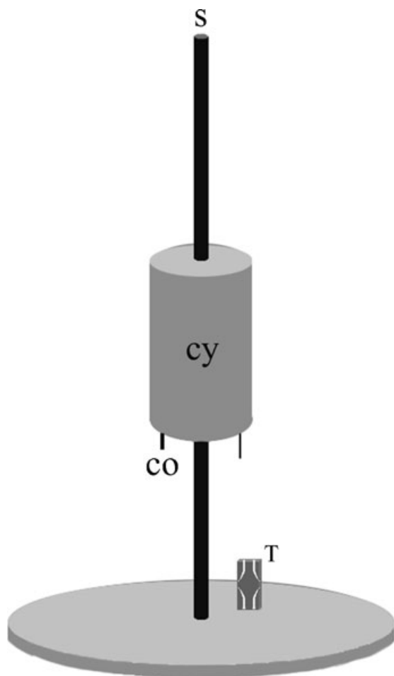
Figure 2 The device used to compact the gutta-percha cones. cy, cylinder; s, shaft; co, compactor tip; T, training block with simulated canals.
