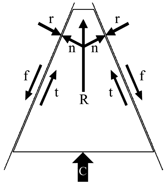
Figure 3 Vectorial decomposition of the compaction force between two inclined planes. C, compaction force that can be decomposed into tangential force (t) and normal force (n). r, reaction force; f, friction force; R, resulting force.
